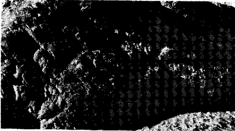
Photo 2 - Basaltic lava flows ( β ), resting on the detrital lacustrine deposits ( plq ) in the south of Bingöl. Further south in this outcrop, the unconsolidated deposits overlie the basaltic lavas.
