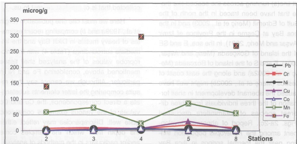
Fig. 4b- Distributions of the abundance of the heavy metal concentrations at the of stations 2, 3, 4 and 8
