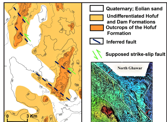
Figure 6- Elevation contours and simplified geological map of the Al Habl region-west of Ghawar area. Offset along the ridges may provide evidence for sinistral movements, on the NW trending fault system, Perinçek et al., 1998b, 2000a-b).
