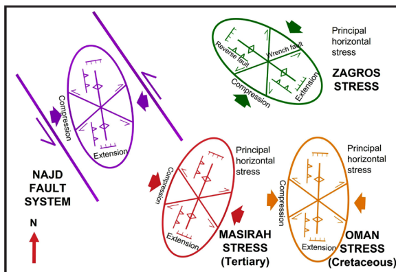
Figure 4- Stress diagram for deformation related to Najd Fault System and Oman, Zagros, Masirah stress regimes.
